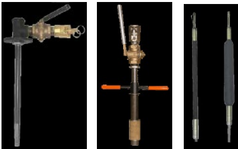
Drive Packer (1), Mechanical Surface Grout Packer (2) and Inflatable Grout Packer (3) shown above
